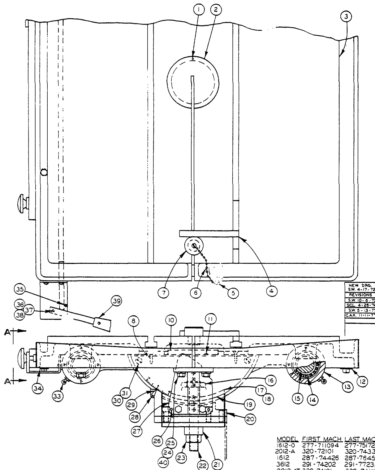
SLIDING TABLE ASS'Y. AIR FEED
