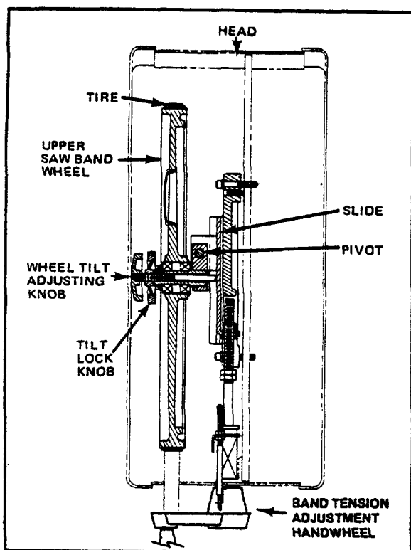
FIG. 10. WHEEL TILT ADJUSTMENT -SIDE VIEW.
