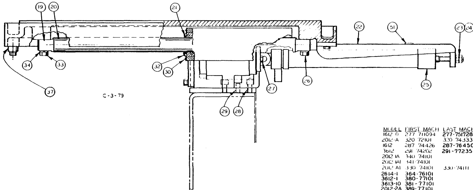
SLIDING TABLE ASS Y AIR FEED
