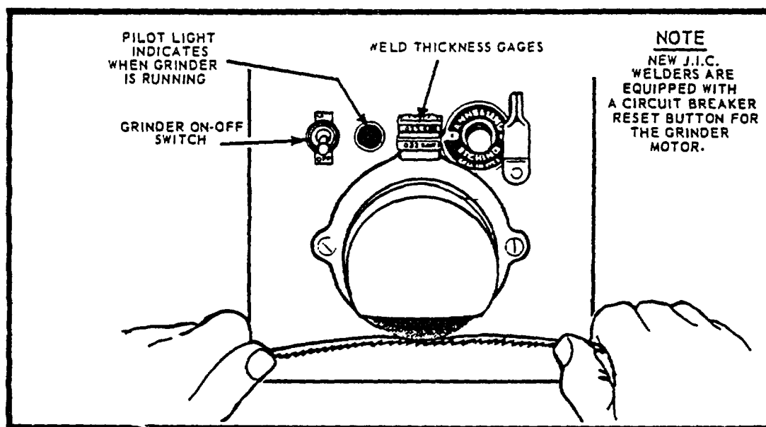
Grinding the weld.
