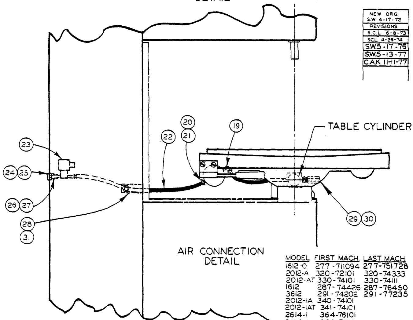
AIR FEED SLIDING TABLE ASS'Y.
