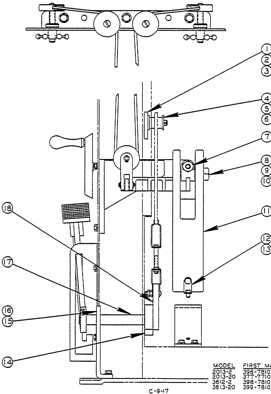
WEIGHT FEED ASSEMBLY (CONTINUED)
