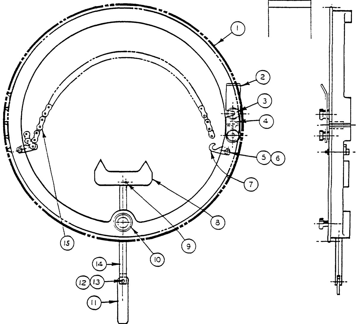
#403310 CONTOUR FEED WORK HOLDING FIXTURE
