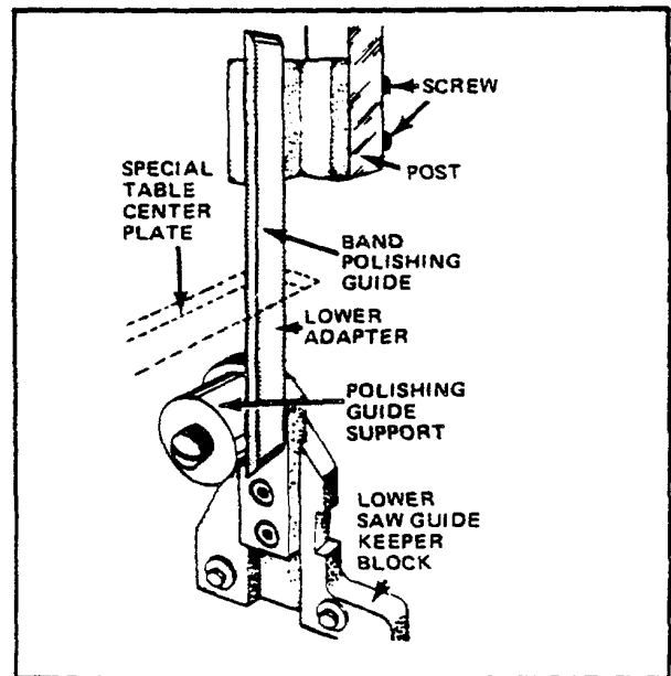
FIG. 49. BAND POLISHING GUIDES.
