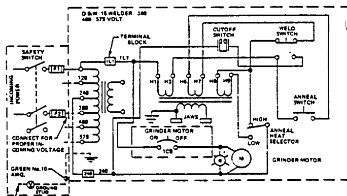
STANDARD DIAGRAM FOR OPERATION ABOVE 240 VAC PORTABLE No. 132817-3
