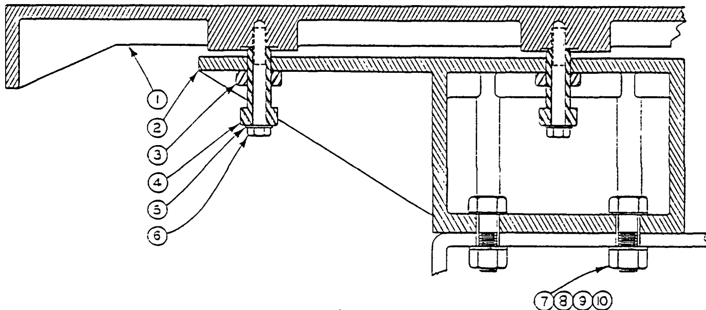
FITS ALL 36" MACHINES #50369 SECONDARY TABLE MOUNTING ASSY C-3-38 CM-3-26
