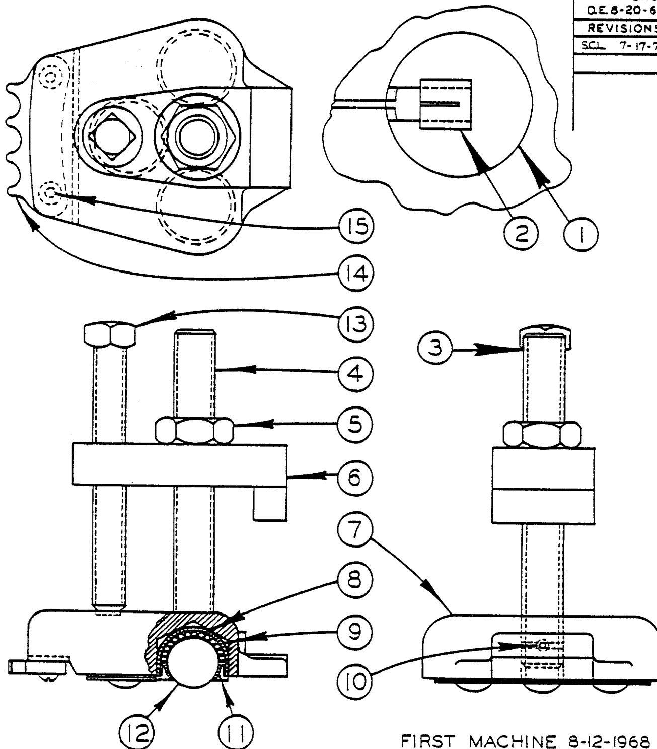
HEAVY PARALLEL WORK CLAMP
