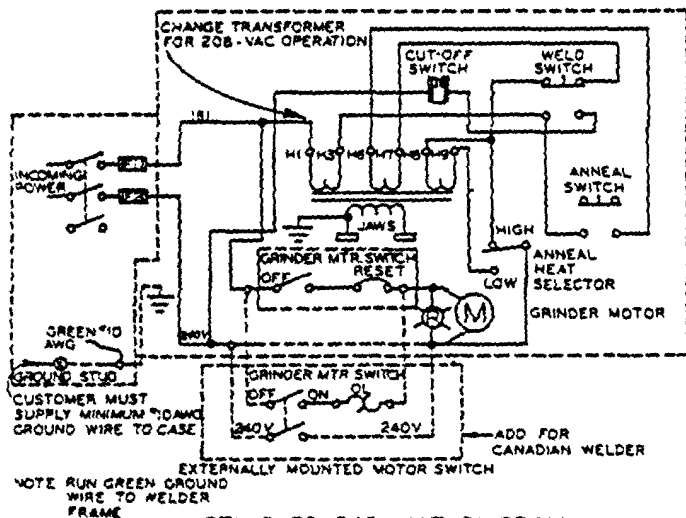
STANDARD 240-VOLT DIAGRAM PORTABLE *132816-2
