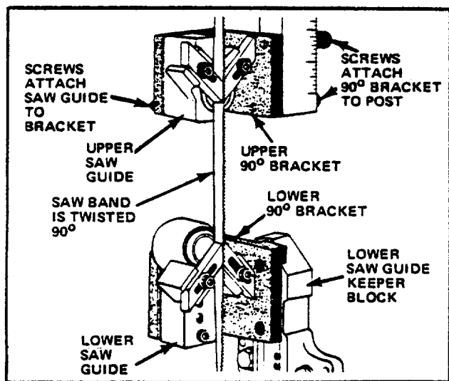
FIG. 28. 90° SAW SAND GUIDE BRACKETS.
