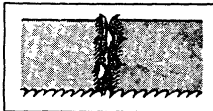
"Blown-out" weld.
