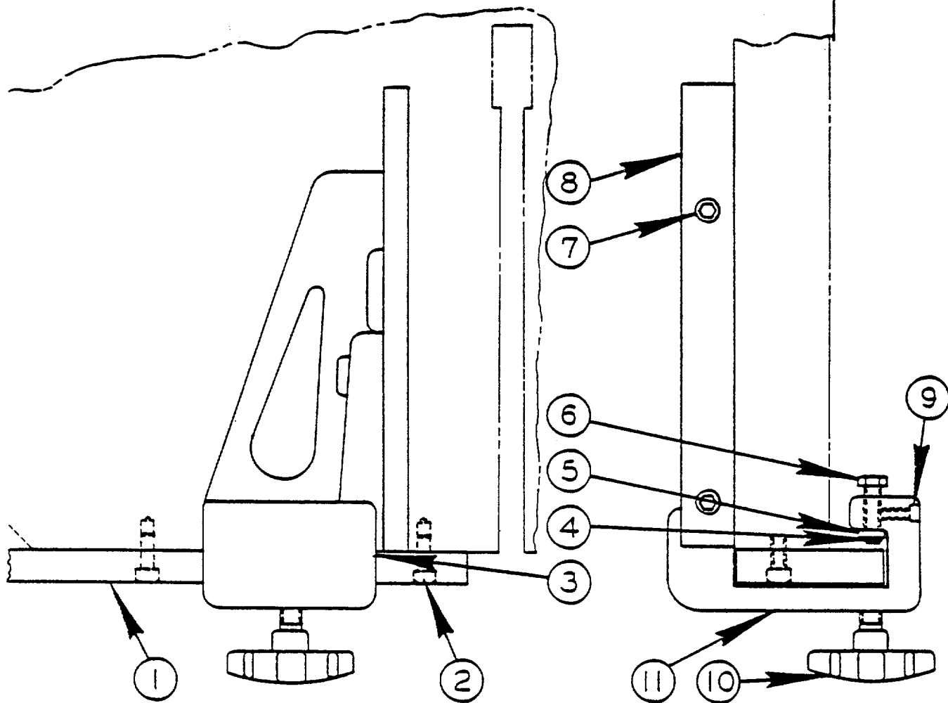
RIP FENCE ASSEMBLY
